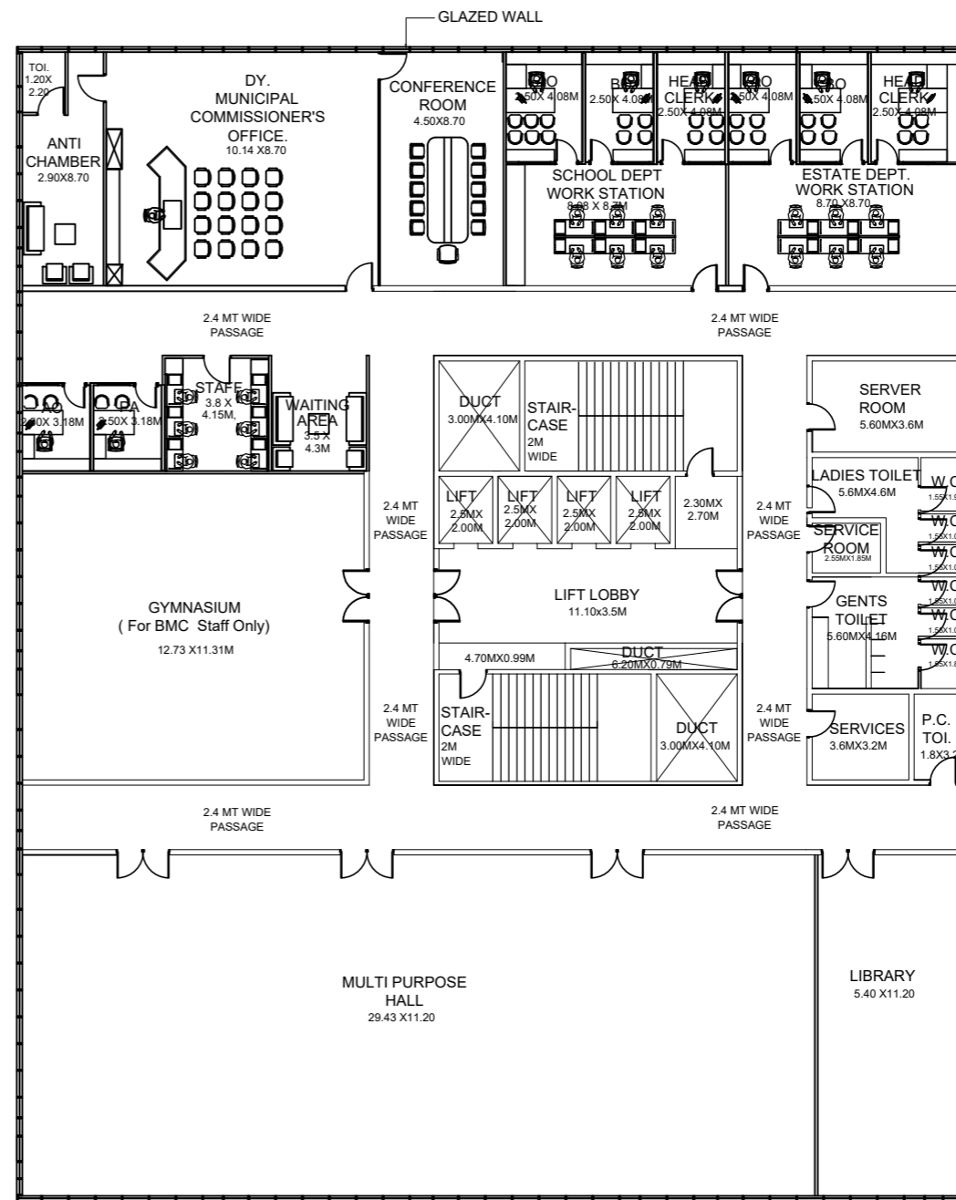
6TH FLOOR PLAN SCALE - 1:100
