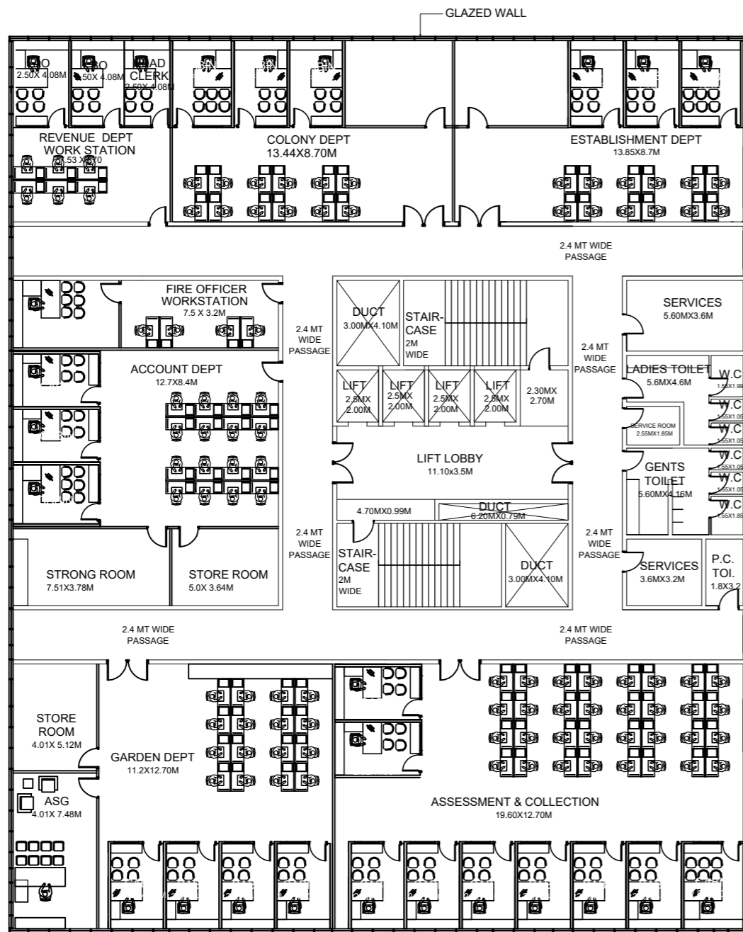
5TH FLOOR PLAN SCALE - 1:100
